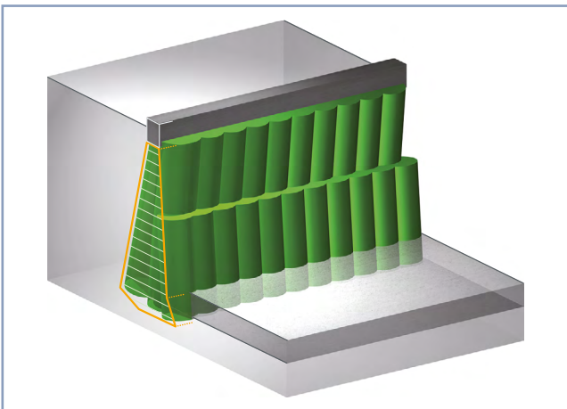
Underpinning elements
