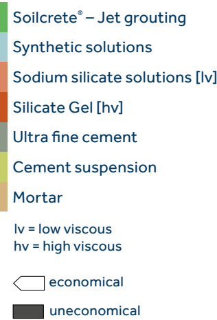
Application limits for grouting techniques
